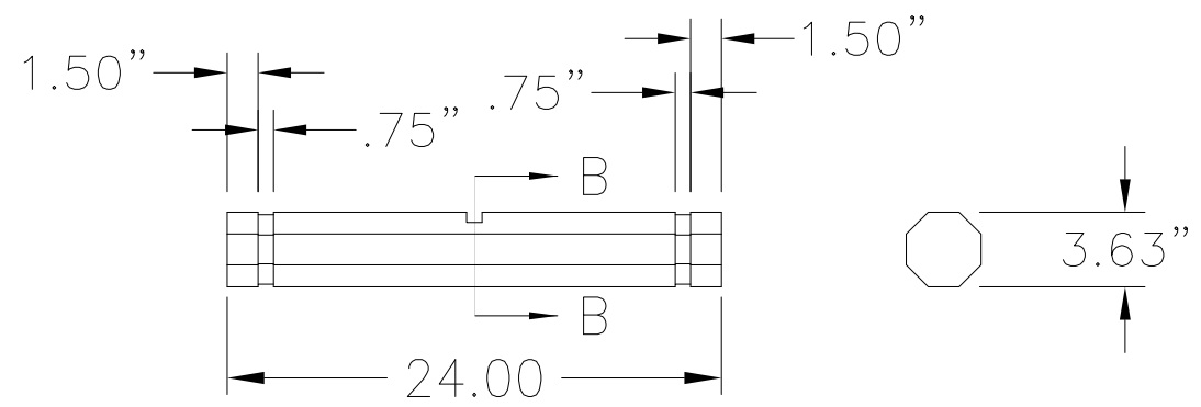
LEG (4 REQD)
